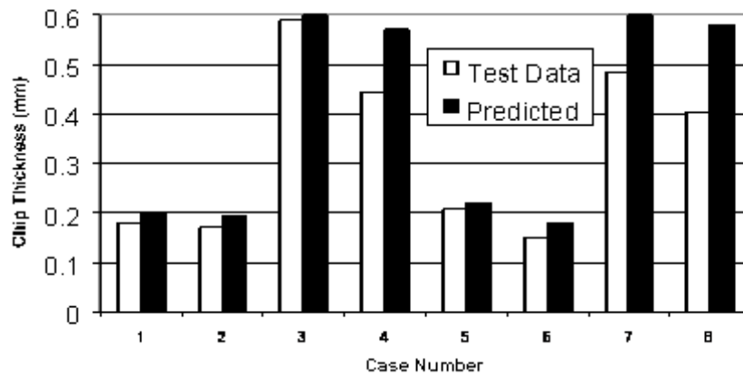
Figure 10 Comparison between predicted and measured chip thickness over a range of cutting conditions for flat rake face cutters.
