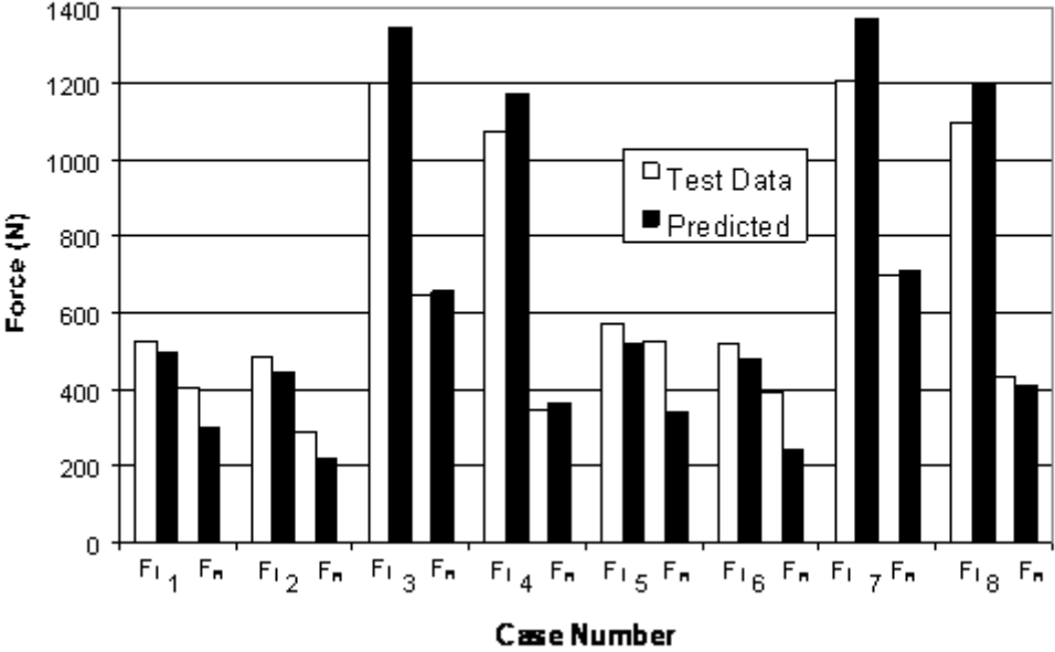
Figure 9 Comparison between predicted and measured force components over a range of cutting conditions for flat rake face cutters.
