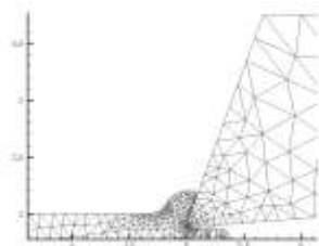
Figure 2 Initial tool indentation
