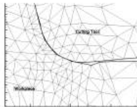
Figure 5 Initial mesh.
