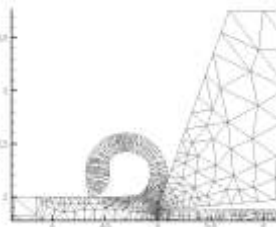
Figure 3 Chip formation
