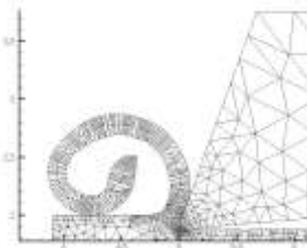
Figure 4 Fully developed continuous chip
