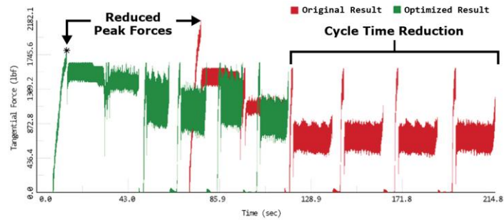
AdvantEdge Production Module balances tool loads and recommends new feeds and speeds, optimizing the user's NC program.
